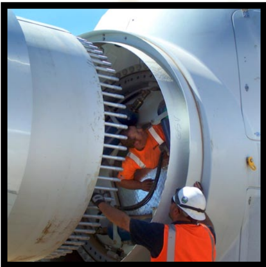
Wind Technicians aligning the bolt fit on wind turbine rotor assembly Photo credit: John Demoss
