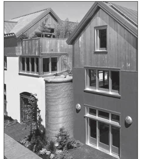
The Watershed is constructed of aerated autoclaved concrete, with additional insulation added around windows, doors and roofs. The heating and cooling system uses ground-source heat pumps, radiant floors, solar thermal collectors, heat recovery ventilators and photovoltaic panels. The outdoor features include native landscaping materials and rainwater collection. Photo courtesy of THE CITY OF EUGENE
